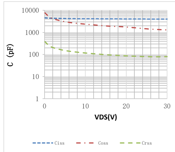
Fig.2 Capacitance Characteristics
